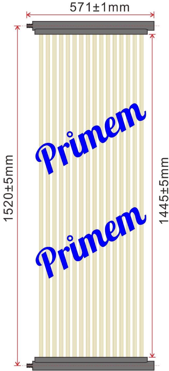
Schematic Drawing
