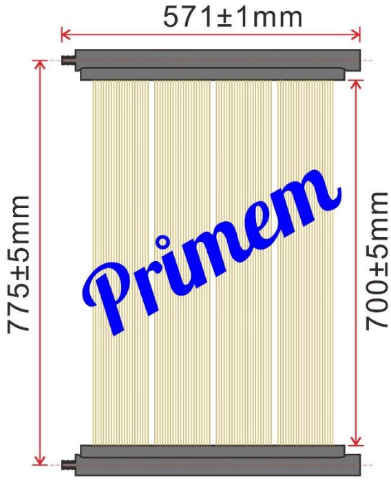
Schematic Drawing
